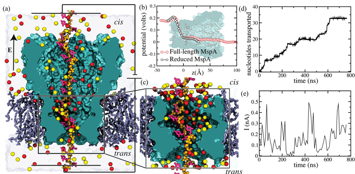
Figure 1. MD simulations of ssDNA transport through MspA. (a) Cut-away view of a full-length MspA system. The MspA nanopore is shown as a teal molecular surface, the POPC lipid bilayer is shown as purple lines, the backbone of a DNA strand threaded through the nanopore is shown as ochre spheres, the DNA bases are shown as thick magenta lines. K^+ and Cl^- ions within a representative 1-nm-thick cross section of the system are shown as red and lemon yellow spheres, respectively. Water is not shown. The locations of the cis and trans sides are specified in the image. (b) Average electrostatic potentials along the symmetry axis of the MspA nanopores at a transmembrane bias of 180 mV. The electrostatic profiles were computed from all-atom MD simulation of open (no DNA) MspA nanopores. In panels a and c, the z axis points normal to the plane of the lipid bilayer. The background image of the nanopore faithfully aligns with the profiles of the electrostatic potential. (c) Cut-away view of a reduced-length MspA system. In the reduced-length MspA system, the DNA strand is covalently joined to itself across the periodic boundary, forming an effectively infinite DNA strand. The coloring scheme is the same as in panel a. (d) The number of cytosine nucleotides translocated through the constriction of the M1 MspA in a typical MD trajectory performed at a 180 mV bias. (e) The ionic current trace for the MD trajectory featured in panel d, sampled at 10 ns.
