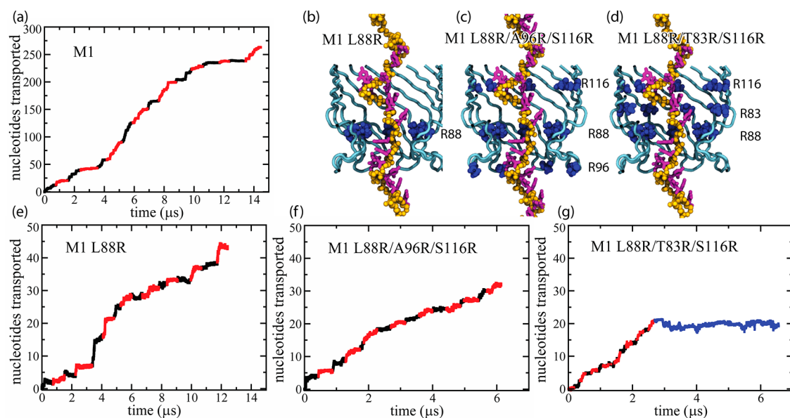
Figure 2. Ensemble simulation of ssDNA transport through mutant variants of MspA. The number of nucleotides translocated through the constriction of MspA at a 180 mV bias is plotted as a function of time for 16 independent systems in the case of (a) M1, (e) M1 L88R, (f) M1 L88R/A96R/S116R, and (g) M1 L88R/T83R/S116R variants of the MspA nanopore and cytosine homopolymers. Each trace is shown in two colors, red and black, indicating multiple trajectories (differing in their initial DNA conformation) that were added consecutively to produce the total permeation trace. In panel g, the last 4- \mu s trace corresponds to a single MD trajectory (blue). Panels b–d show the locations of the arginine residues (blue vdW spheres). The backbone of the DNA strand is shown as yellow spheres with the DNA bases depicted by thick magenta lines.
