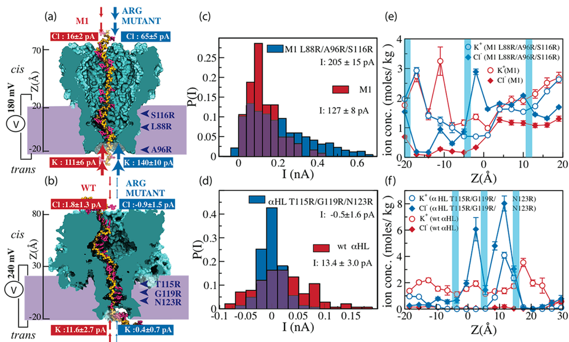
Figure 4. The effect of arginine mutations on the ionic current. (a,b) Cut-away view of the MspA (a) and \alpha HL (b) nanopores containing a DNA strand. The locations of arginine substitutions are indicated by horizontal blue arrows. Simulated values of the K^+ and Cl^- currents at a 180 mV (MspA) or 240 mV ( \alpha HL) bias are specified in the figure. (c, d) Histograms of ionic current obtained from ensemble simulations of the MspA nanopores (c) and single trajectories of the \alpha HL systems (d). The overlap of the two histograms is shown in purple. The histograms were constructed using 100 (MspA) and 1 ( \alpha HL) ns averages of instantaneous current. (e, f) Local concentration of K^+ and Cl^- ions along the symmetry axis of the MspA (e) and \alpha HL (f) nanopores. The blue bars indicate the location of the arginine residues in the nanopores; the z coordinate is defined in panels a and b. The local ion concentration is expressed in molals to avoid uncertainties associated with defining the local volume of a nanopore containing a strand of DNA.
